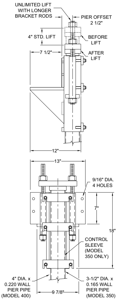
Model 350 & Model 400 Utility Bracket Details
