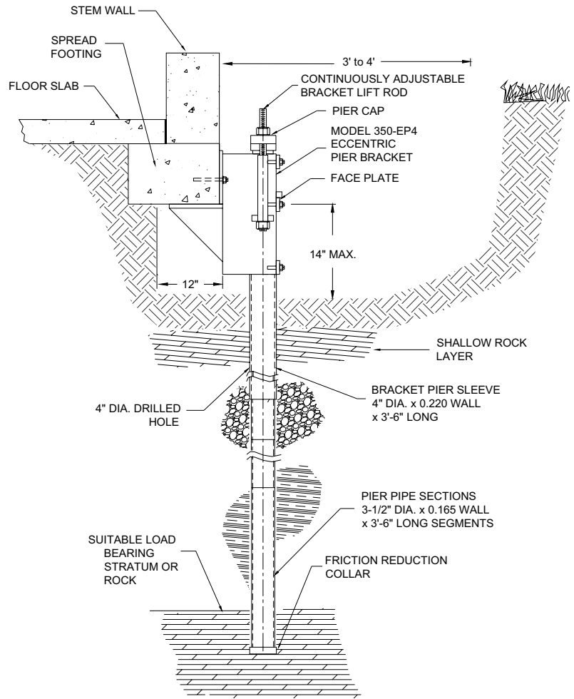
Model 350-EP4 - 4" Eccentric Utility Bracket Application Drawing
