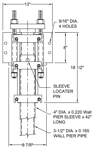
Model 350-EP2 - 2" Eccentric Utility Bracket Details
